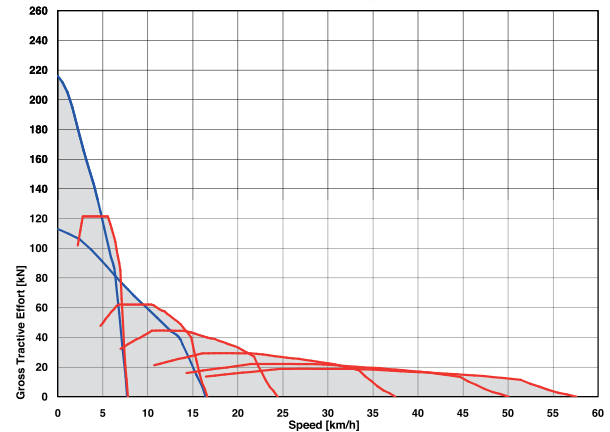
ADT, B30E 6X6 - Tractive Effort
