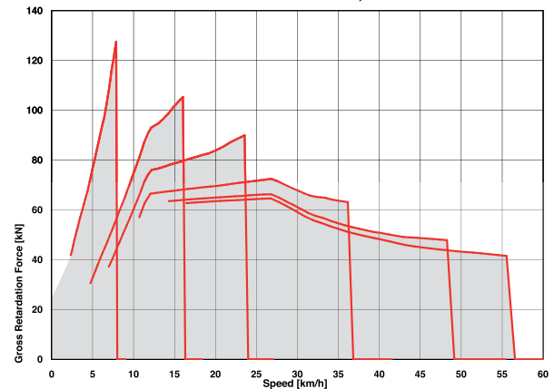
ADT, B30E 6X6 - Retardation
